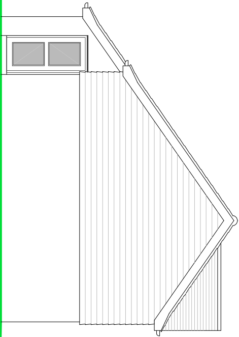
SIDE ELEVATION
