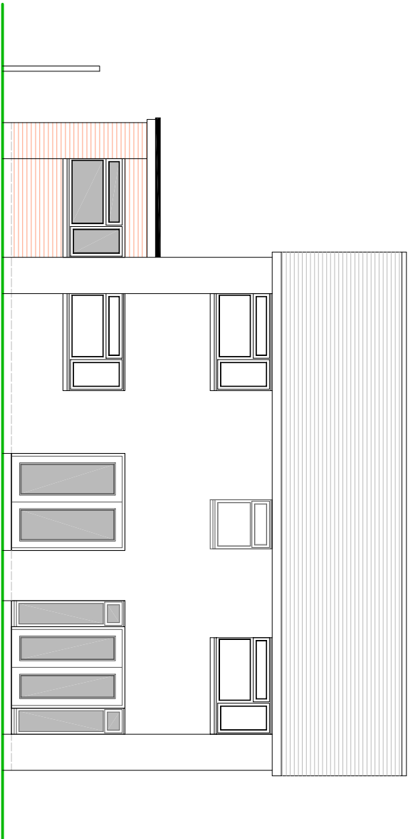
REAR ELEVATION
