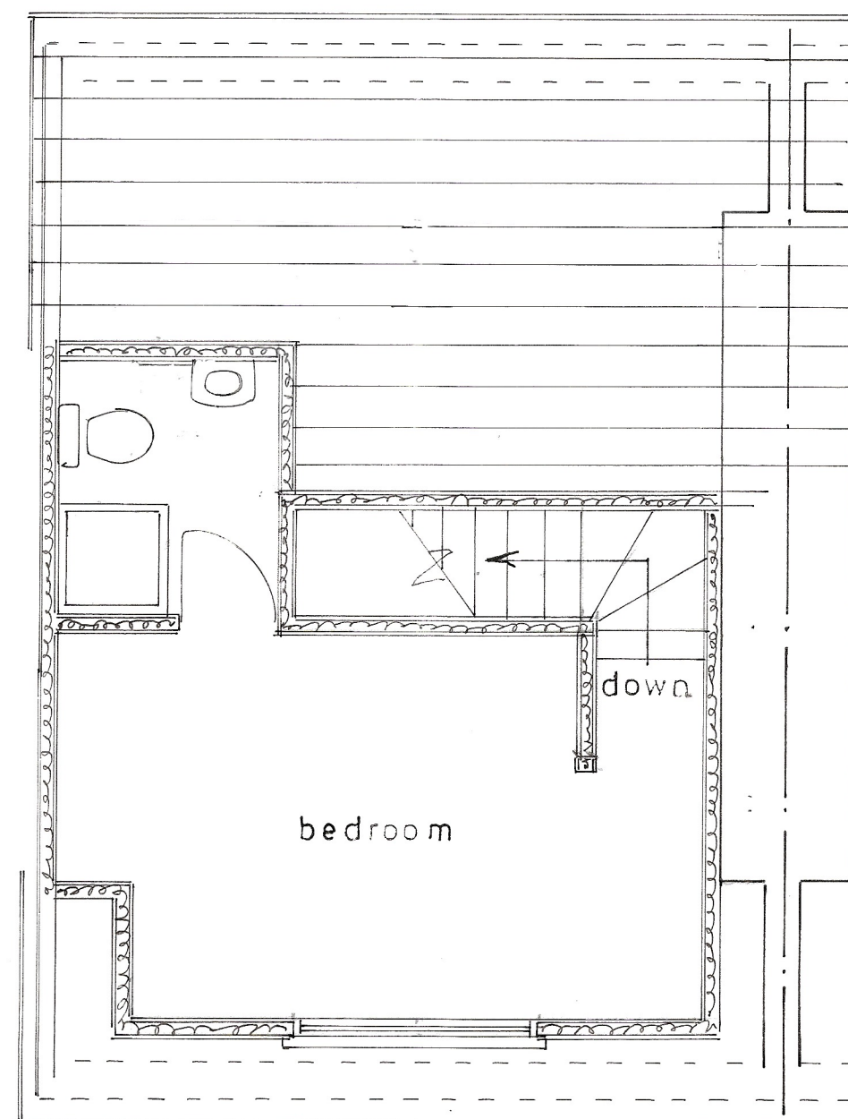
2nd floor plan 1 : 50
