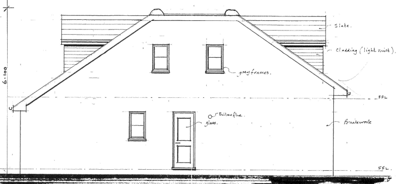
North Elevation
