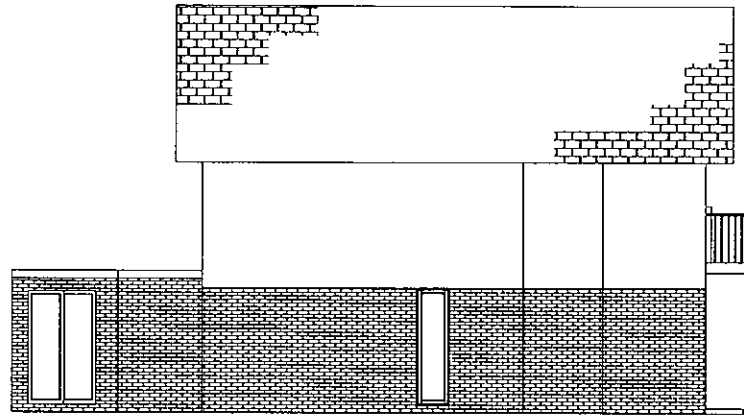
WEST ELEVATION
