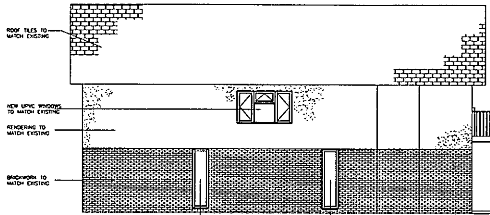
EAST ELEVATION
