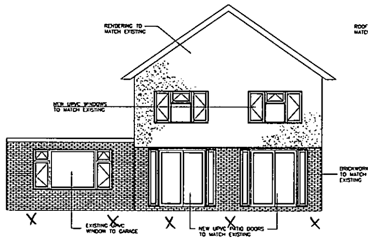
SOUTH ELEVATION
