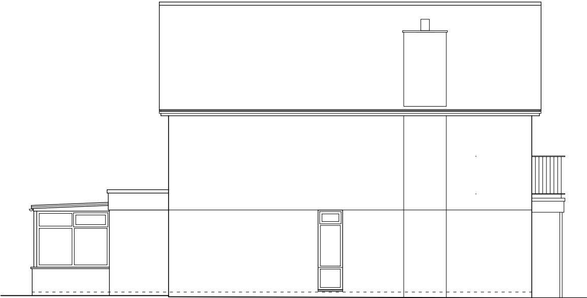
West Elevation
