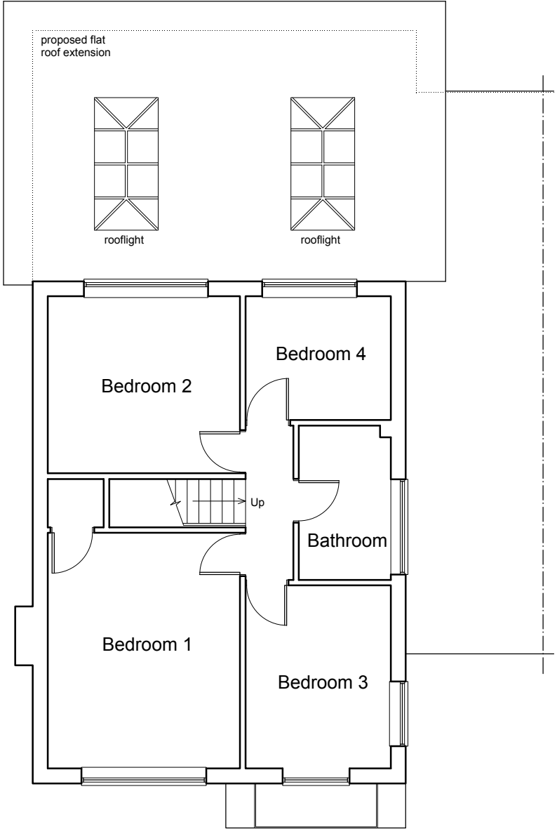
First Floor / Roof Plan
