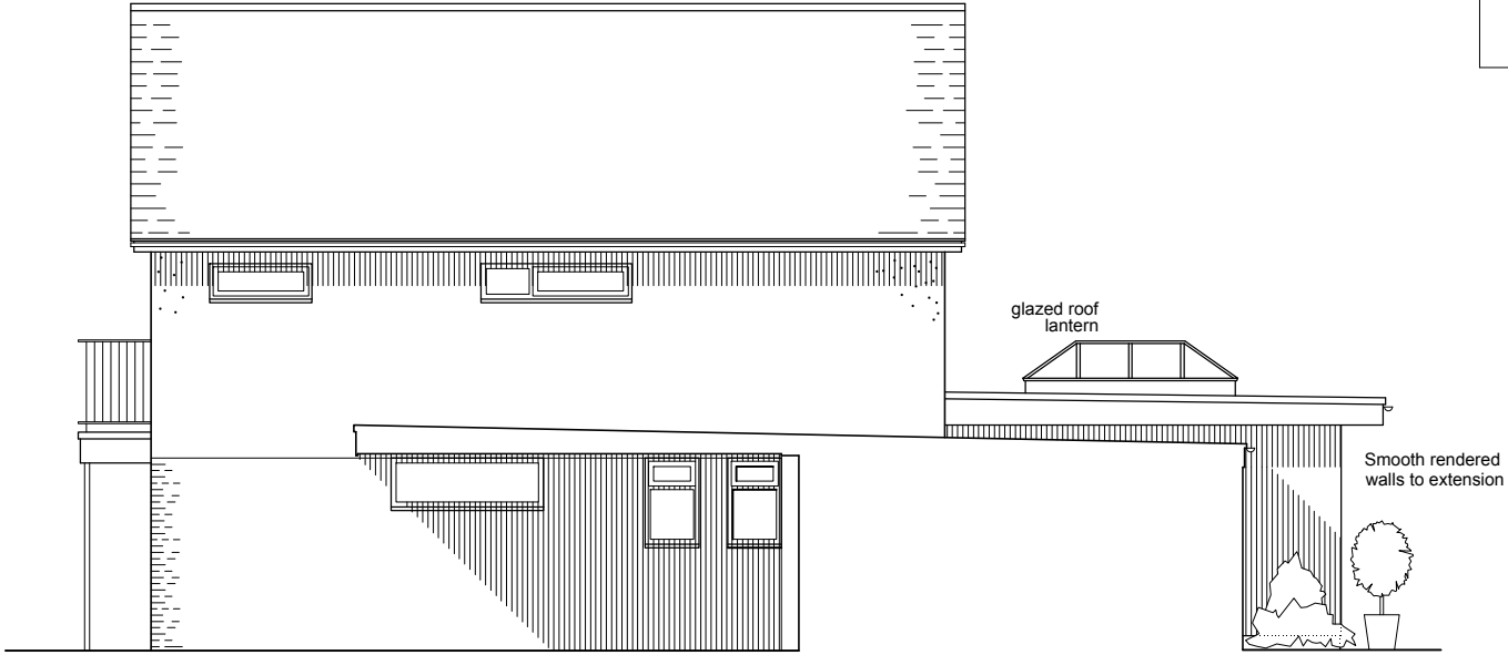
East Elevation
