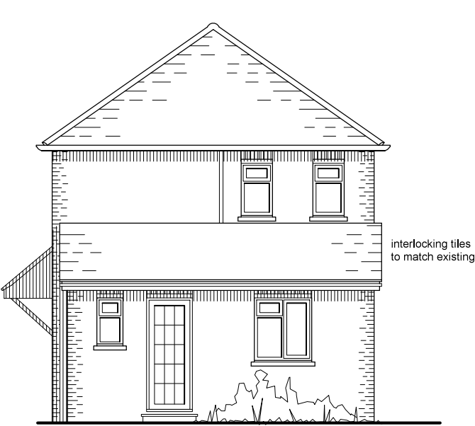
North Elevation
