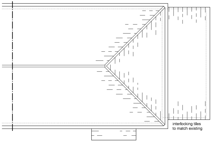
Roof Plan
