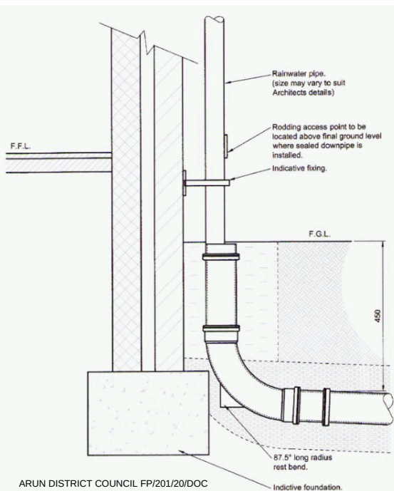
DETAIL OF RAINWATER PIPE (Scale 1:20)
