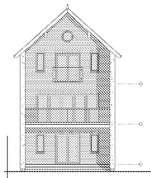
SOUTH ELEVATION
