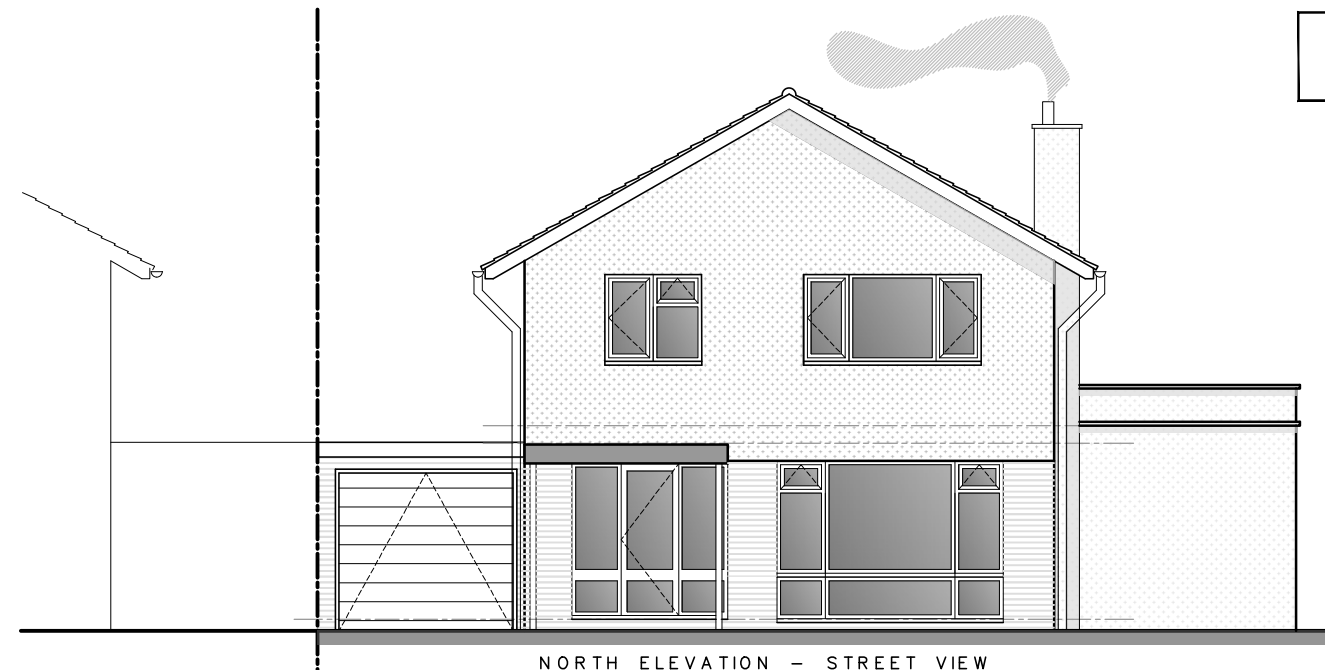
NORTH ELEVATION – STREET VIEW (SCALE 1:100)
