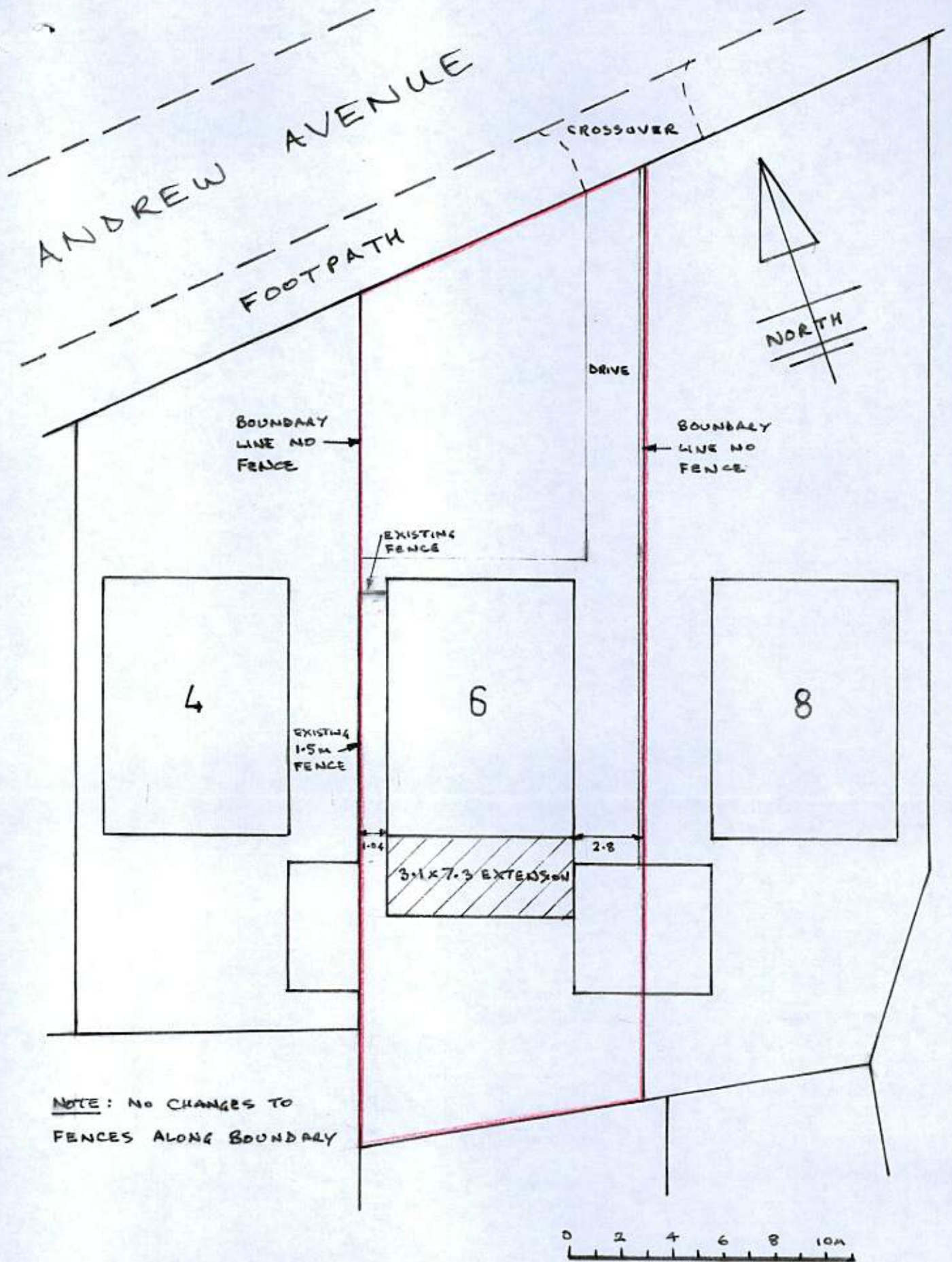
BLOCK PLAN SCALE: 1 200 6 ANDREW AVENUE BOGNOR REGIS
