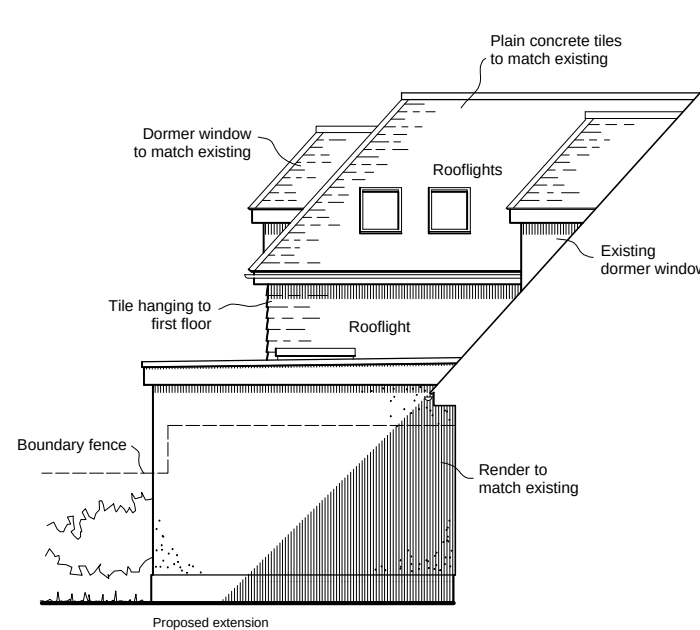
South Elevation
