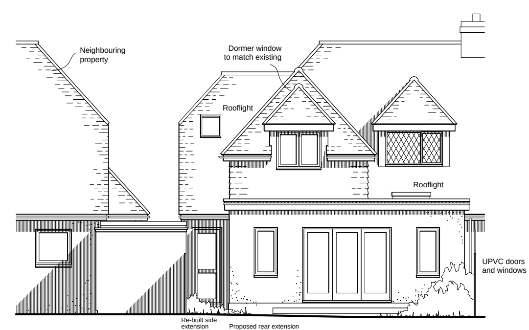
West Elevation
