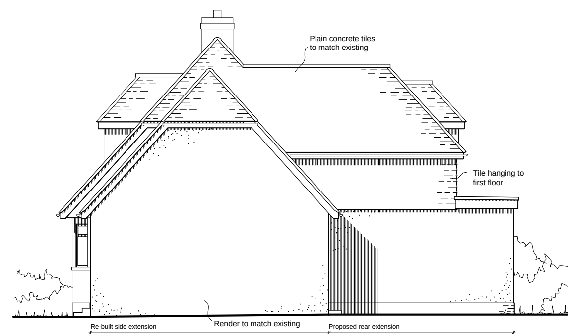
North Elevation
