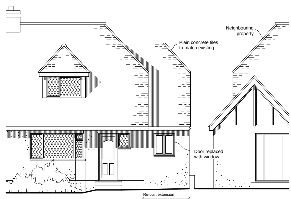
East Elevation
