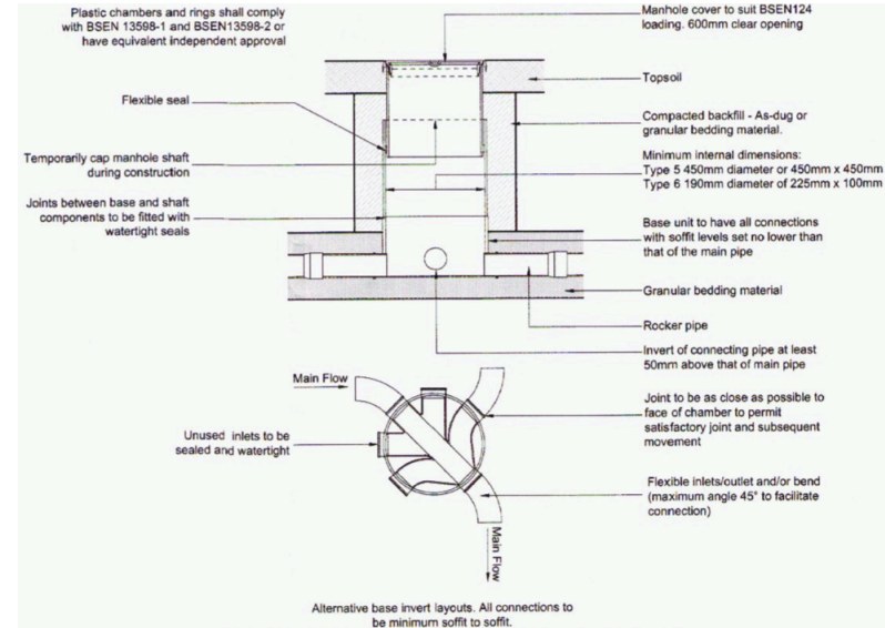
TYPICAL ACCESS CHAMBER DETAIL- TYPES 5 & 6 (LANDSCAPED AREAS) 1m MAXIMUM DEPTH TO FROM COVER TO PIPE SOFFIT. (NON ENTRY) LOCATED IN LANDSCAPED AREAS
