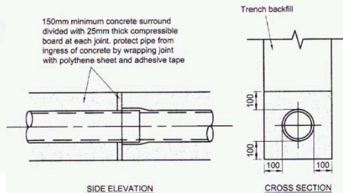
CONCRETE BED AND SURROUND TO PIPES UNDER DRIVES AND GARDENS
