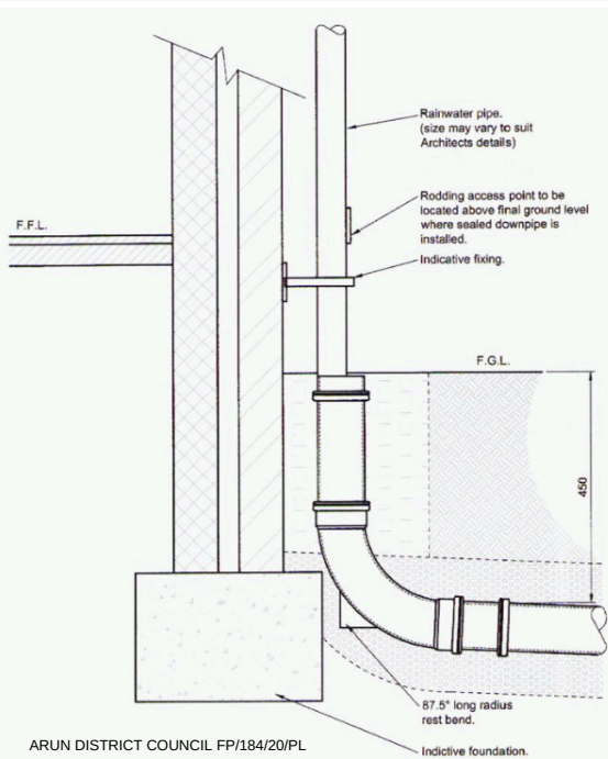
DETAIL OF RAINWATER PIPE (Scale 1:20)
