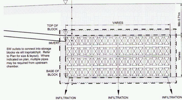
TYPICAL AQUACELL SOAKAWAY (pedestrian and car/light van loading only). (Scale 1:20)
