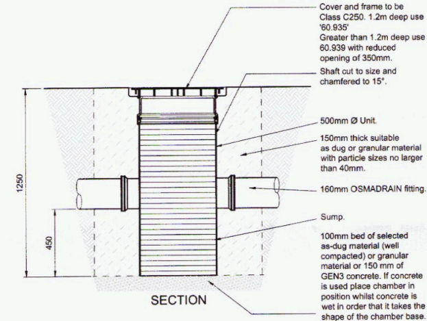
POLYPROPYLENE SHALLOW SILT TRAP DETAIL (500Ø) (Scale 1:20)
