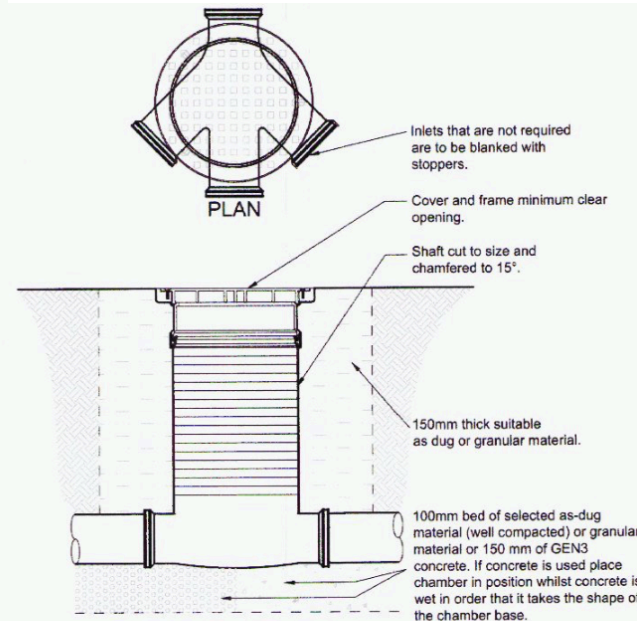
SECTION POLYPROPYLENE SHALLOW INSPECTION CHAMBER DETAIL (250Ø) (Scale 1:20) Depth to invert of less than 600mm.
