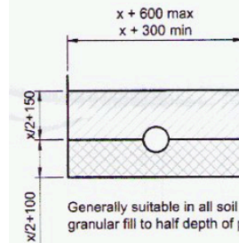
PIPE BEDDING DETAIL UNDER DRIVES AND GARDENS
