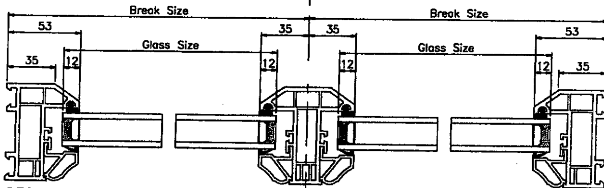
SECTION C-C
