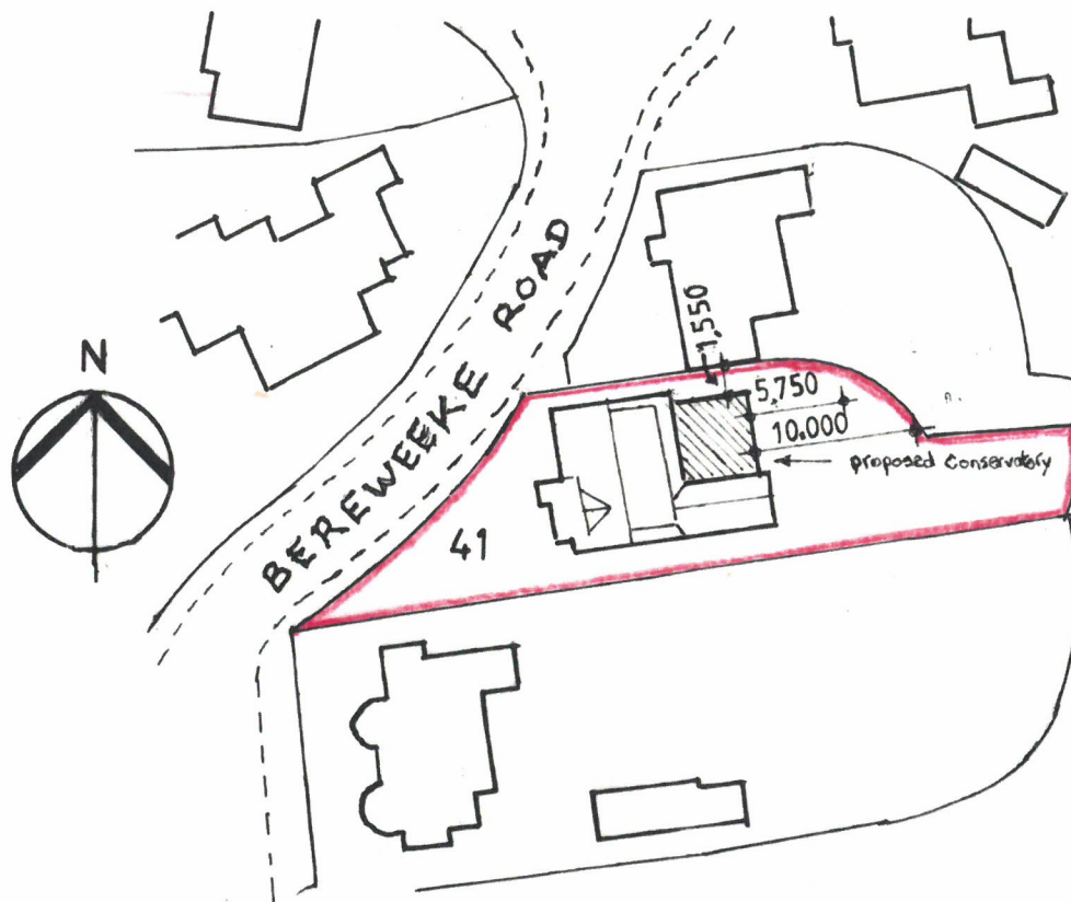
BLOCK PLAN 1:500
