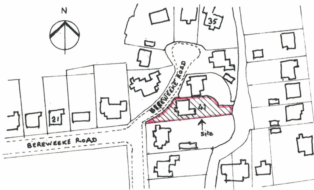
LOCATION PLAN 1:1250
