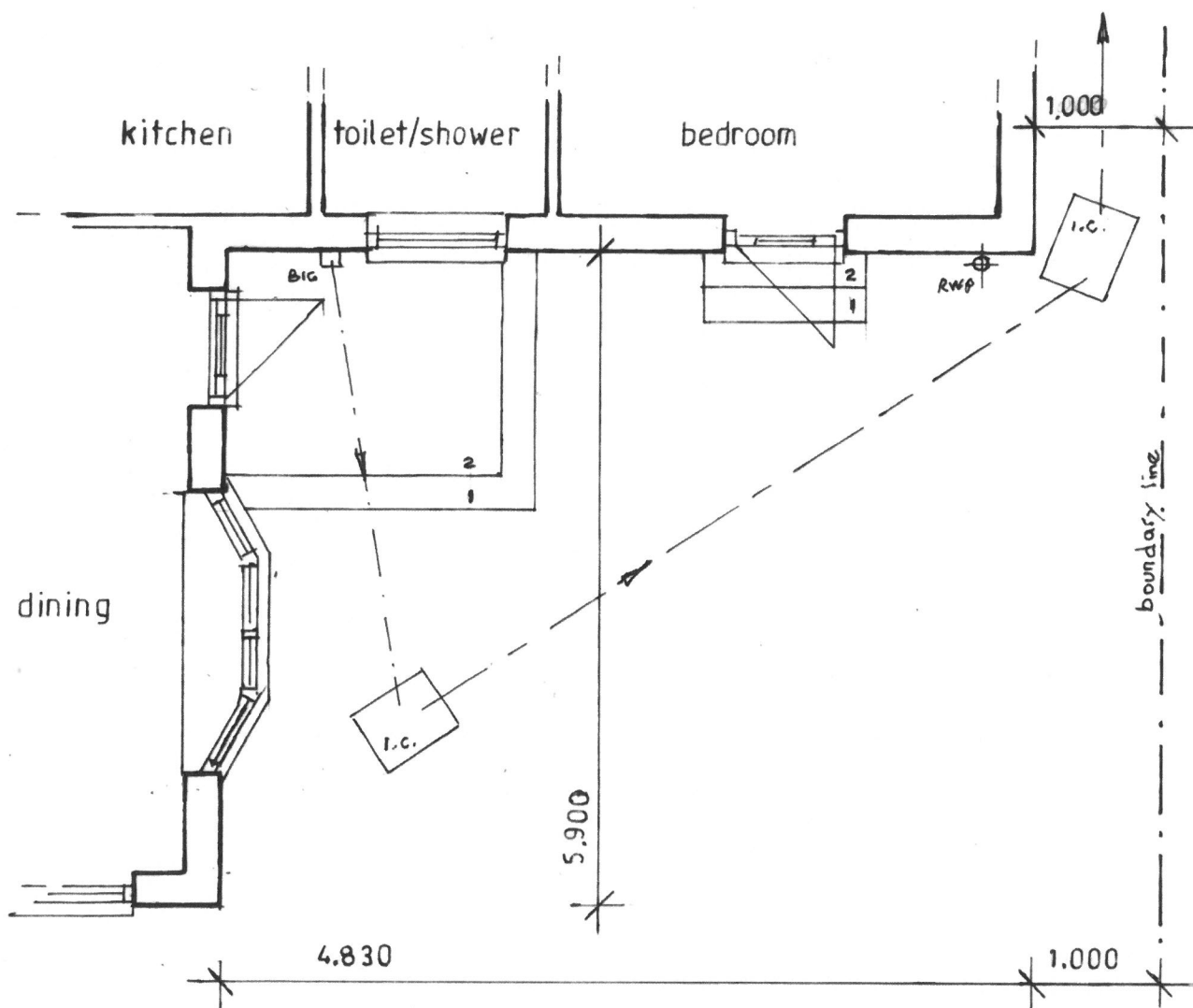
GROUND FLOOR PLAN - AS EXISTING 1:50
