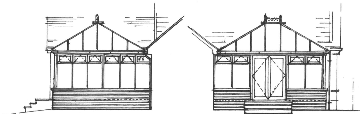
SOUTH ELEV. AS PROPOSED 1:100
