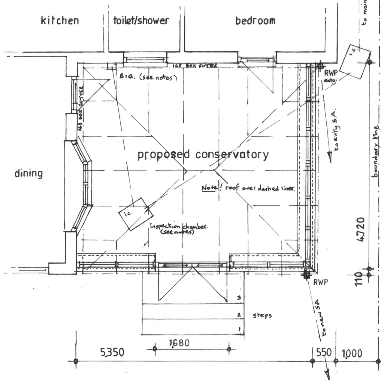
GROUND FLOOR PLAN — AS PROPOSED 1:50
