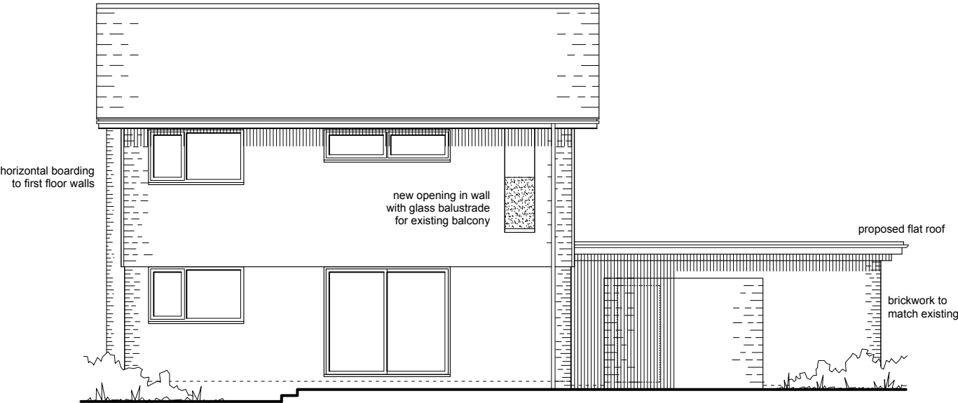
East Elevation
