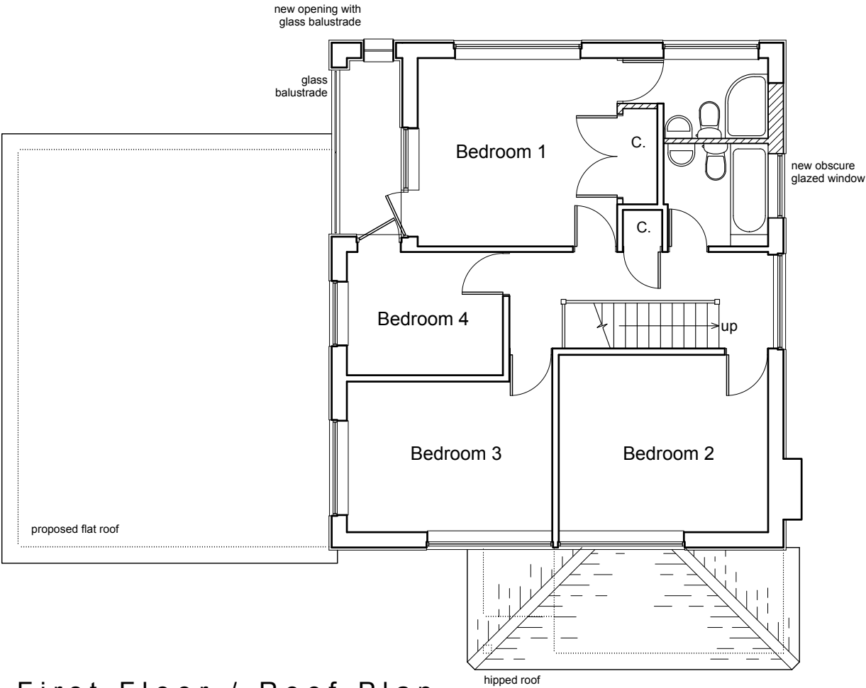
First Floor / Roof Plan
