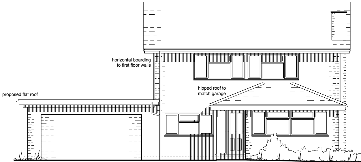
West Elevation
