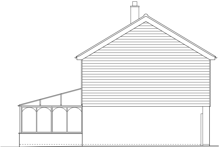
North Elevation
