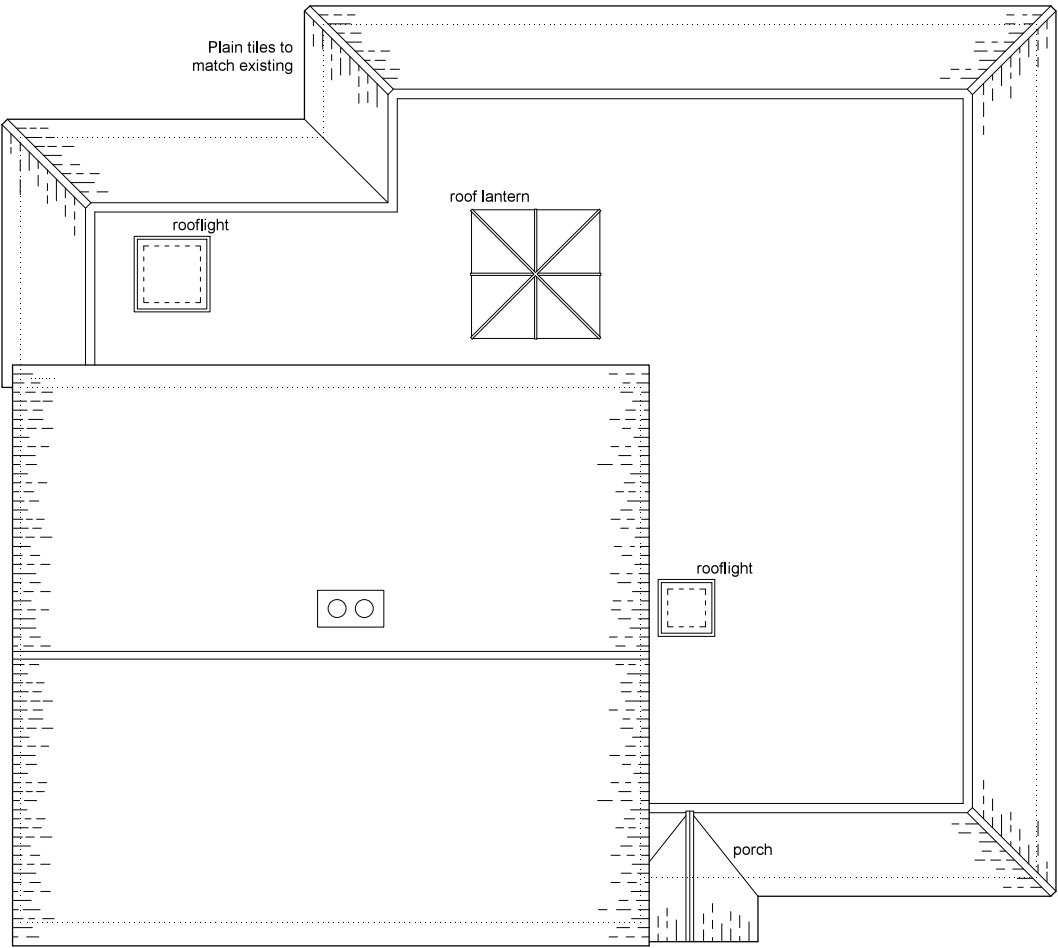
Roof Plan
