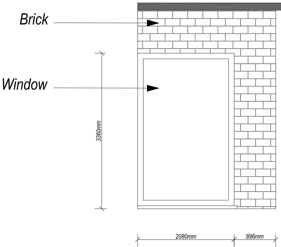
ELEVATION C
