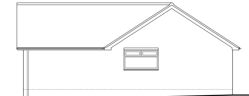
South Elevation
