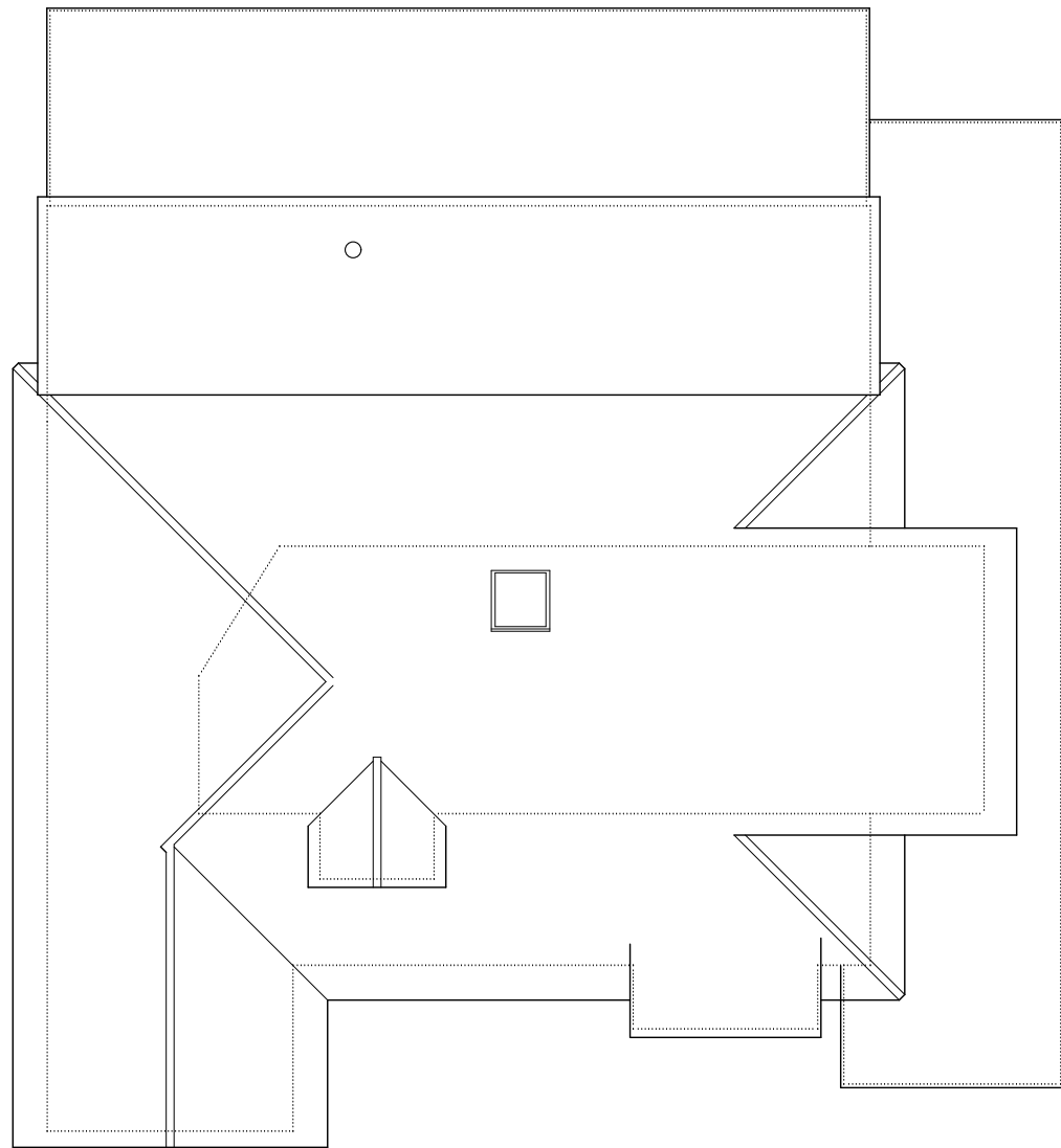
Roof Plan
