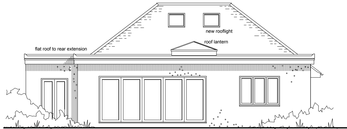
North Elevation
