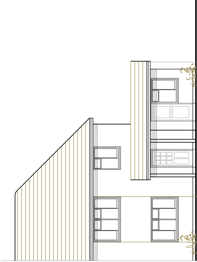
PROPOSED EAST ELEVATION 1:100
