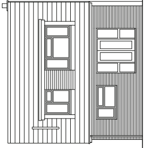
REAR (East) ELEVATION
