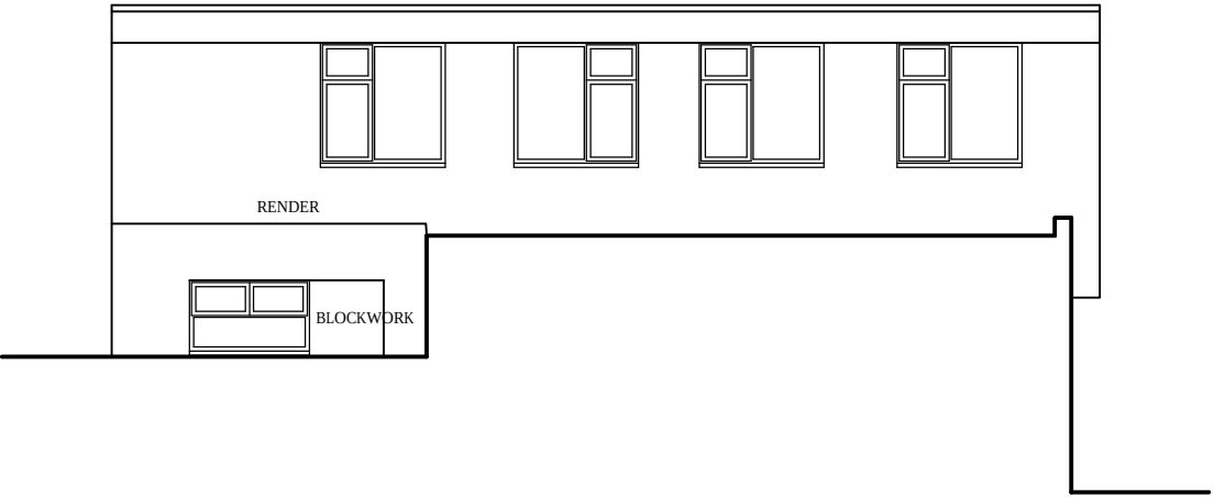
NORTH ELEVATION
