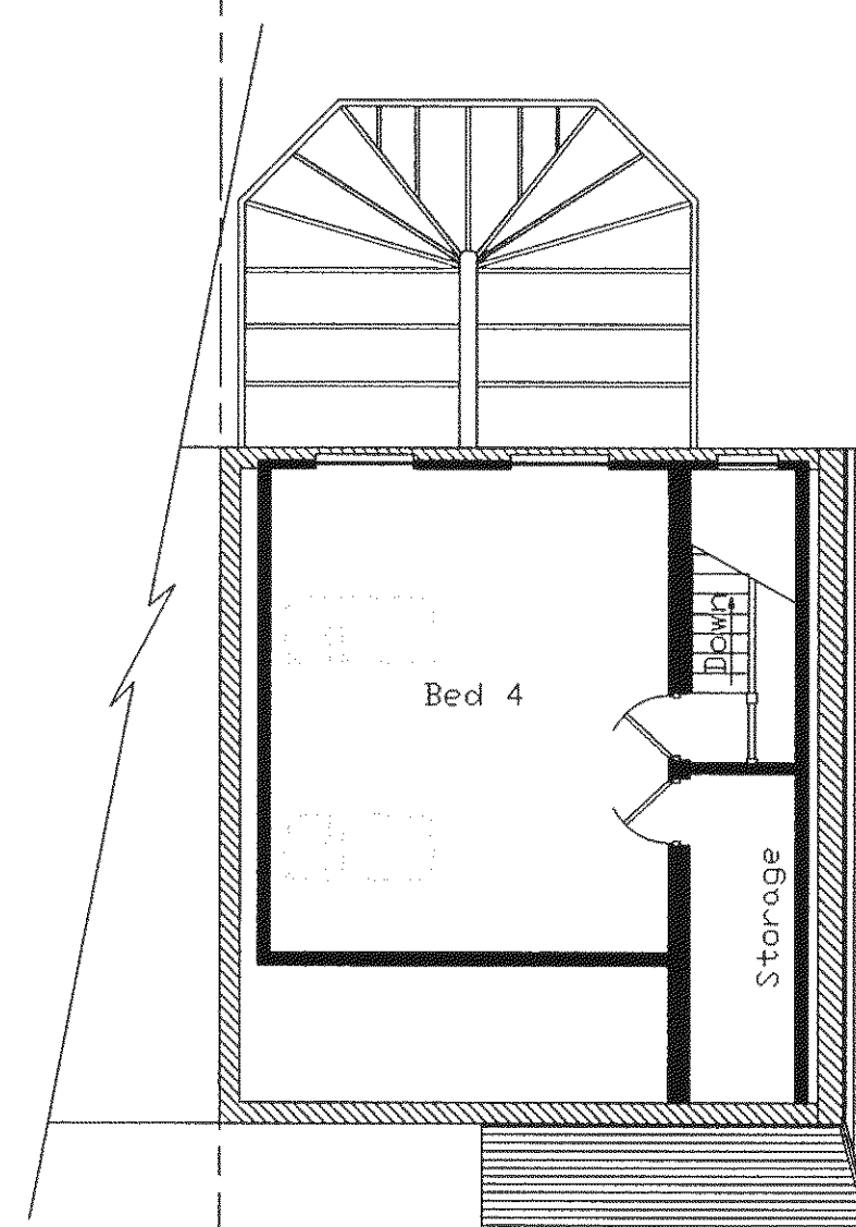
Proposed Loft Room Plan
