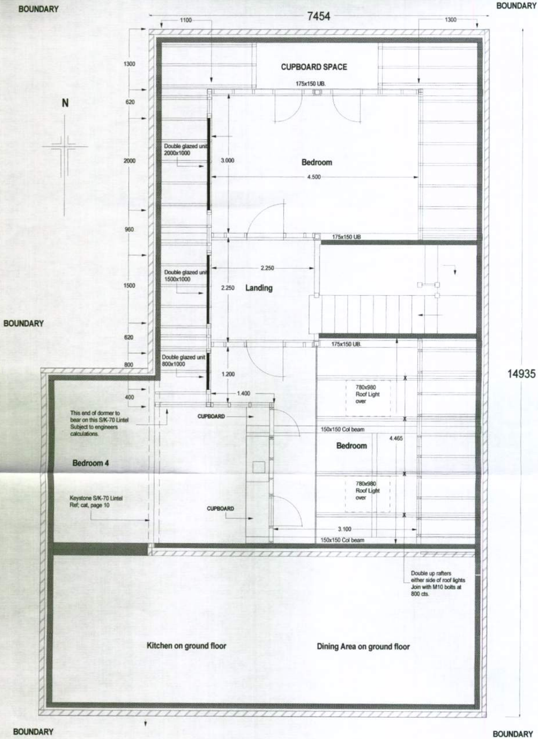
FLOOR AREA, STUD WALLS & WINDOW POSITIONS
