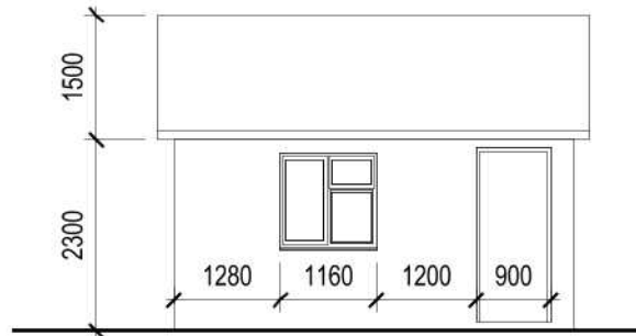
1 North Elevation 1 : 100
