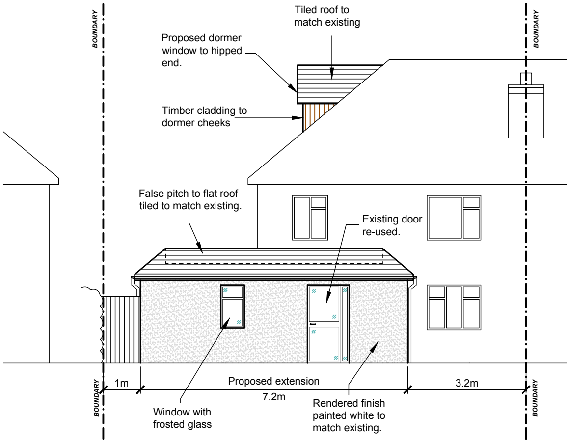
East Elevation - Proposed (1:100)
