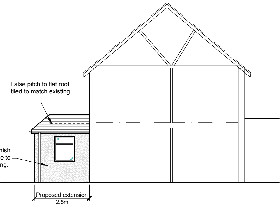
North Elevation - Proposed (1:100)
