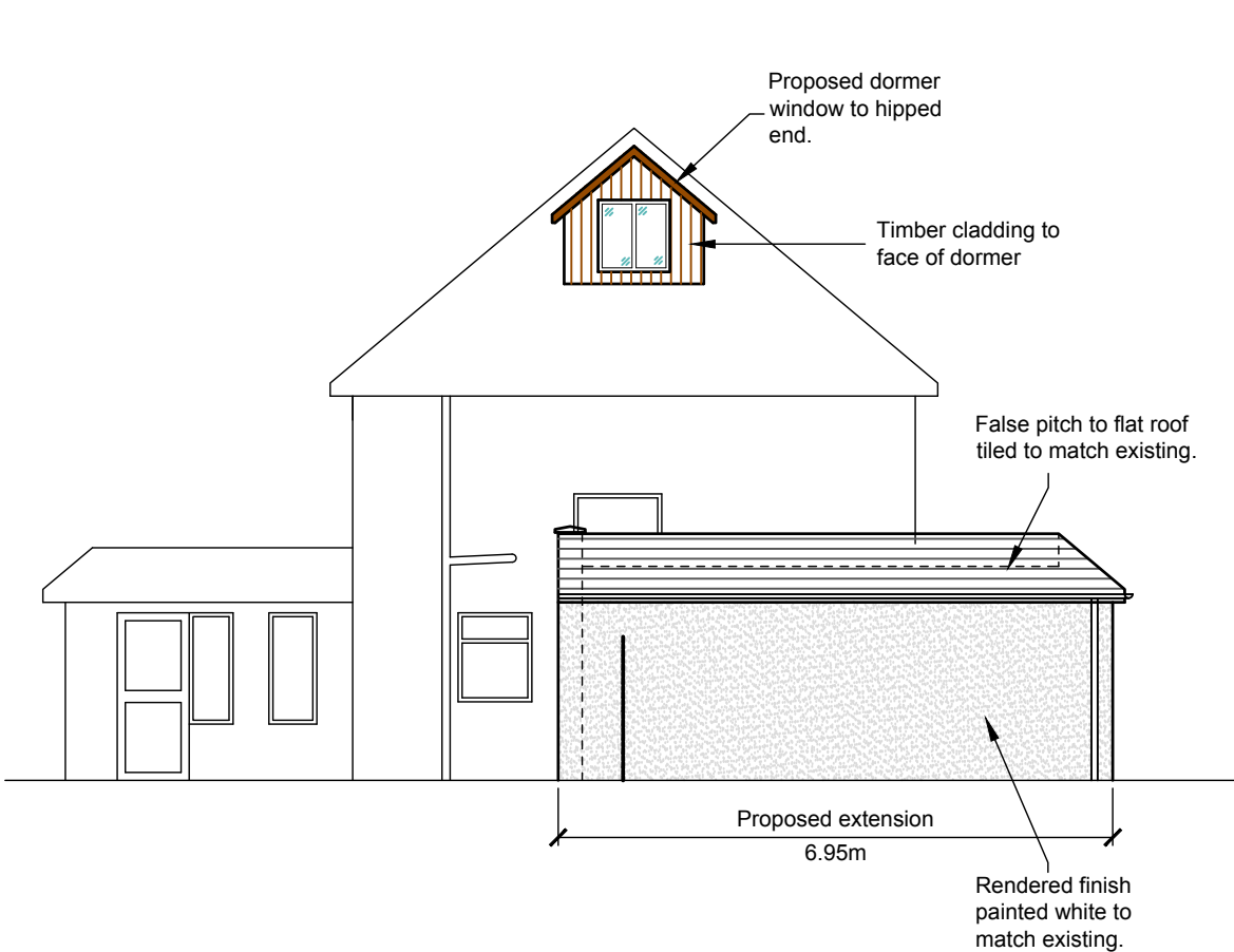
South Elevation - Proposed (1:100)
