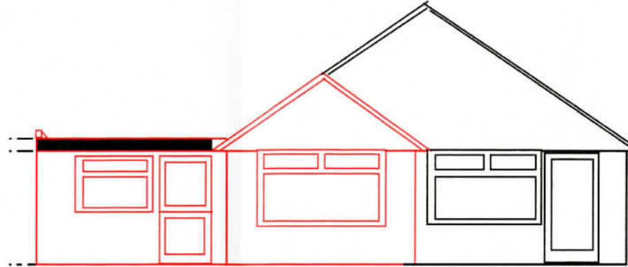
West elevation (rear) proposed
