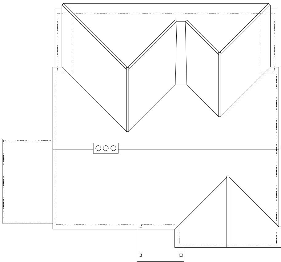
Roof Plan
