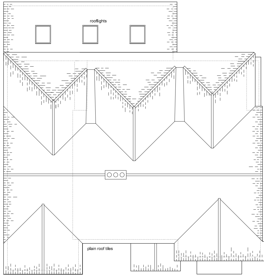
Roof Plan
