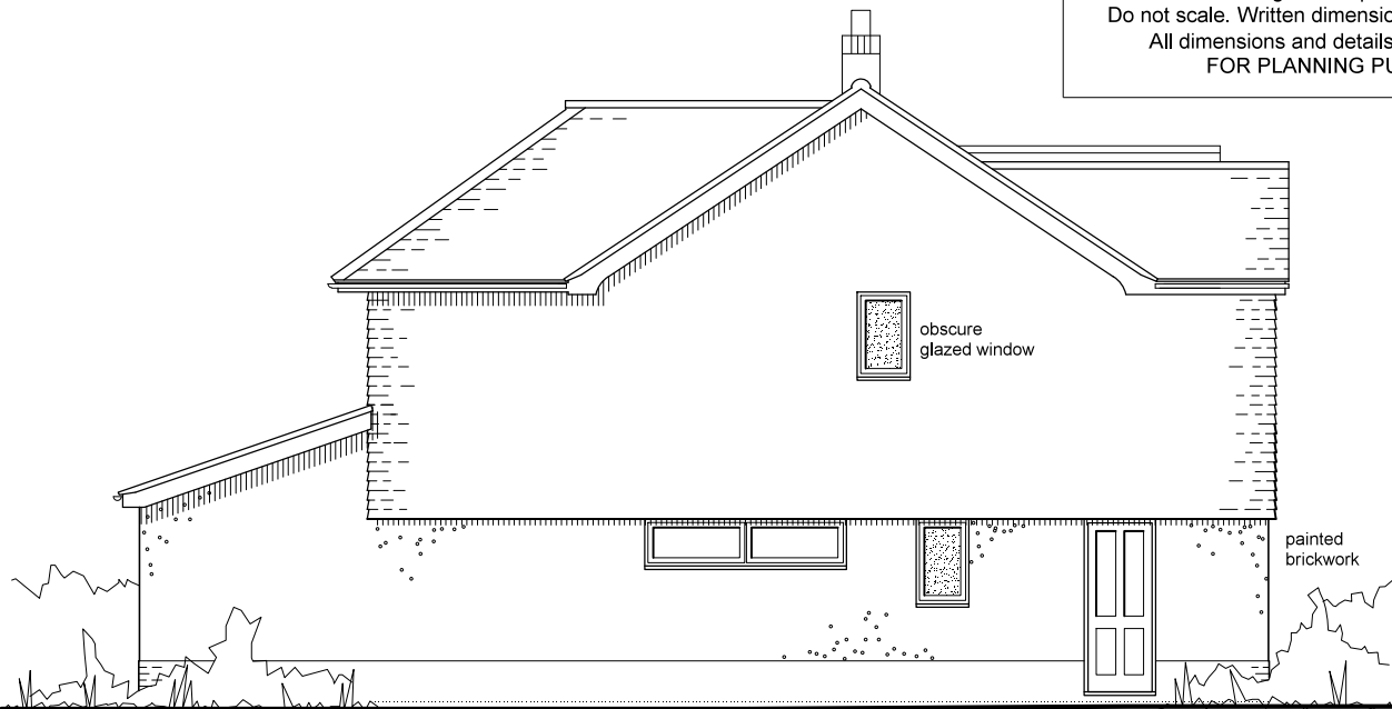
South Elevation
