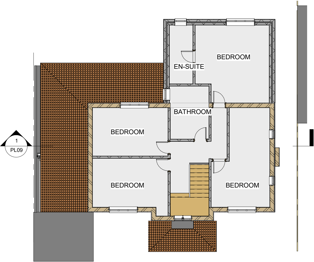
FIRST FLOOR 1 : 100
