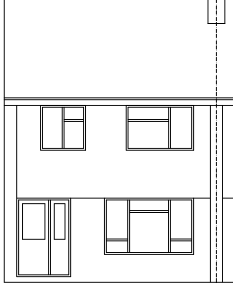
EXISTING NORTH ELEVATION
