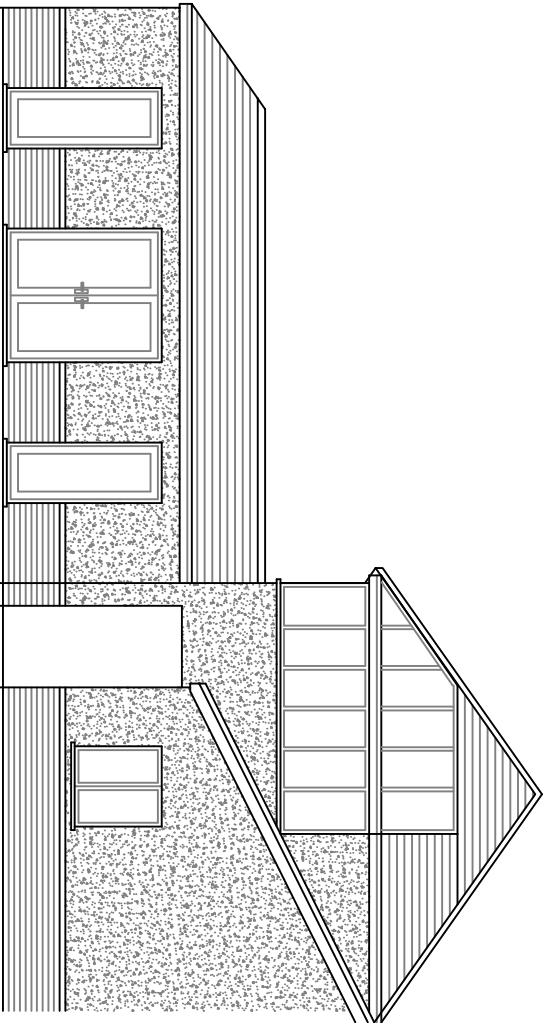
Part Proposed South Elevation
