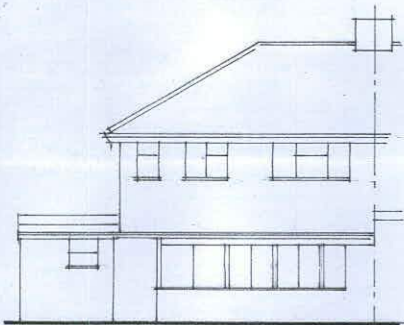
REAR ELEVATION - SOUTH
