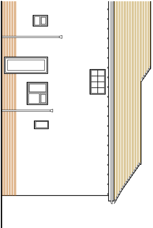
EXISTING PART SIDE ELEVATION
