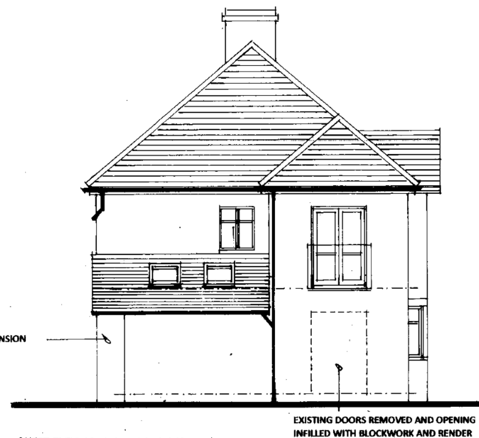
WEST ELEVATION TO GARDENS
