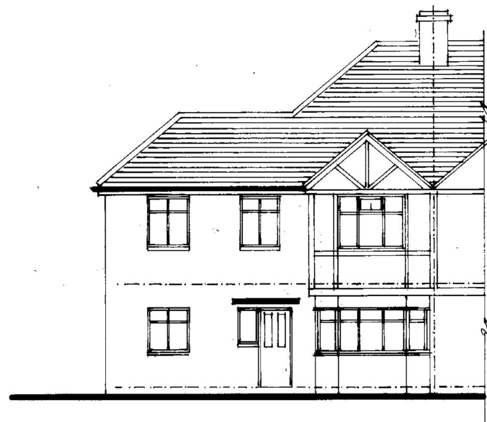
SOUTH ELEVATION TO VICARAGE LANE
