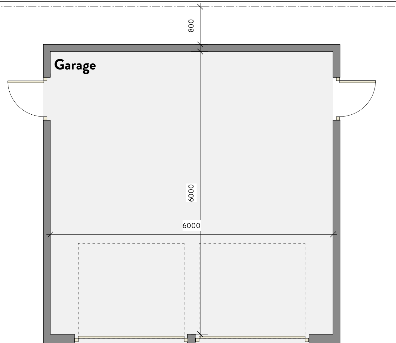
Proposed Plan
