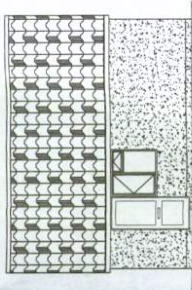
NEW GARAGE NORTH ELEVATION
