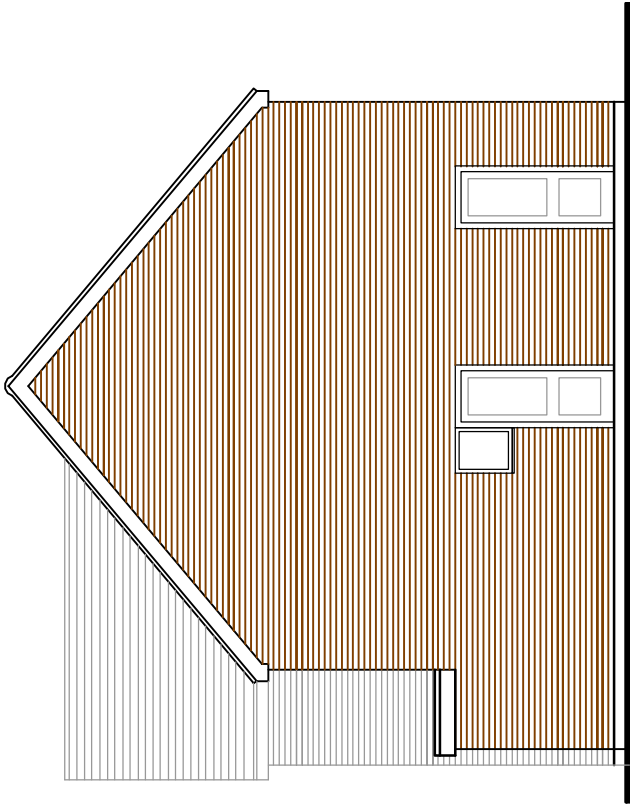
EXISTING SOUTH ELEVATION 1:100
