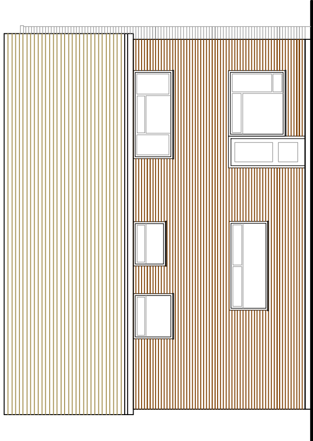
EXISTING EAST ELEVATION 1:100
