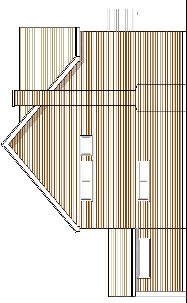
PROPOSED NORTH ELEVATION 1:100
