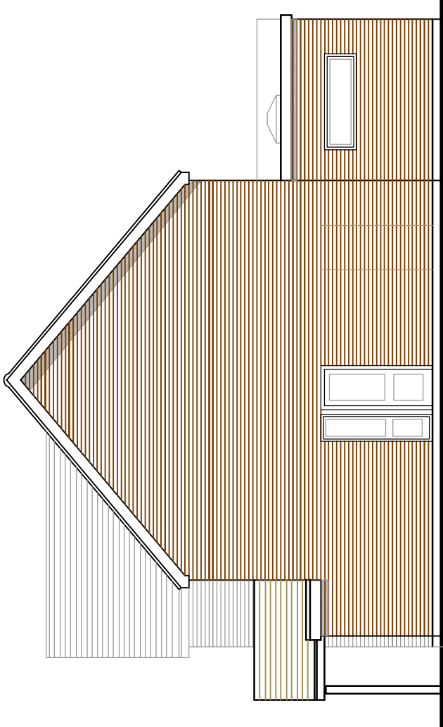
PROPOSED SOUTH ELEVATION 1:100
