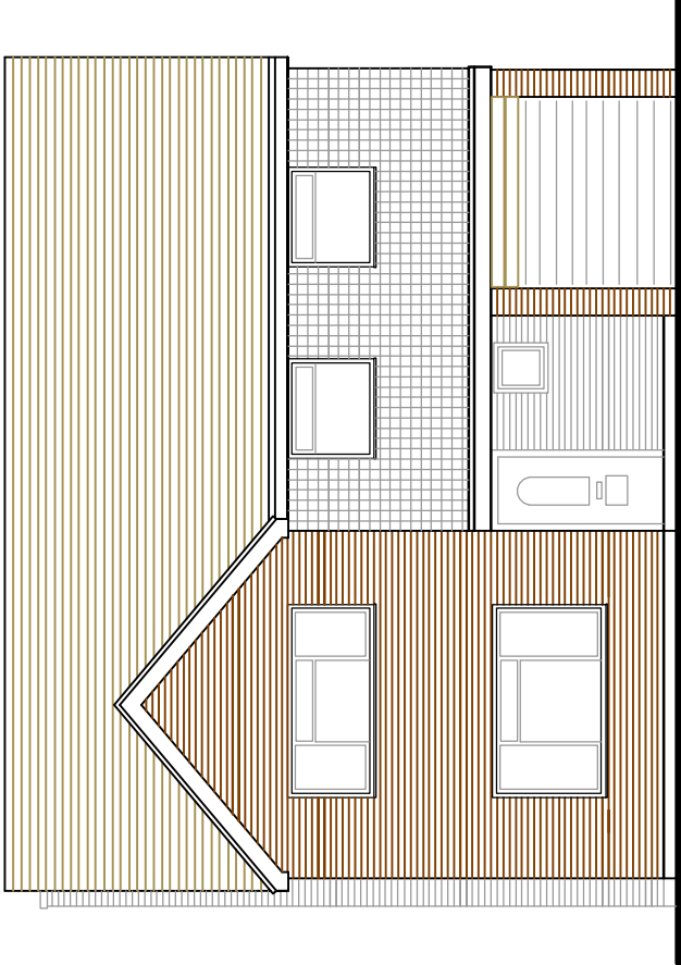
EXISTING WEST ELEVATION 1:100
