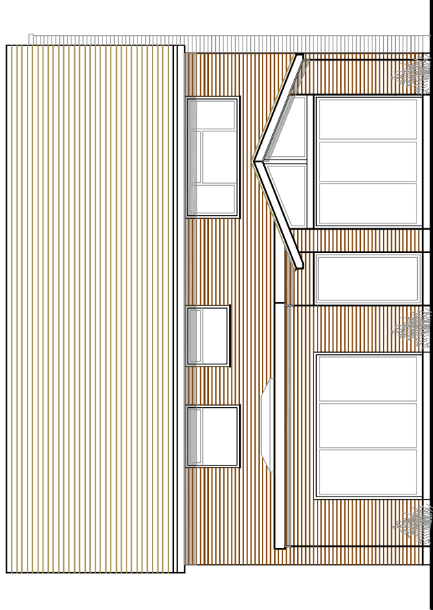
PROPOSED EAST ELEVATION 1:100
