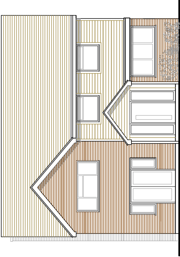
PROPOSED WEST ELEVATION 1:100
