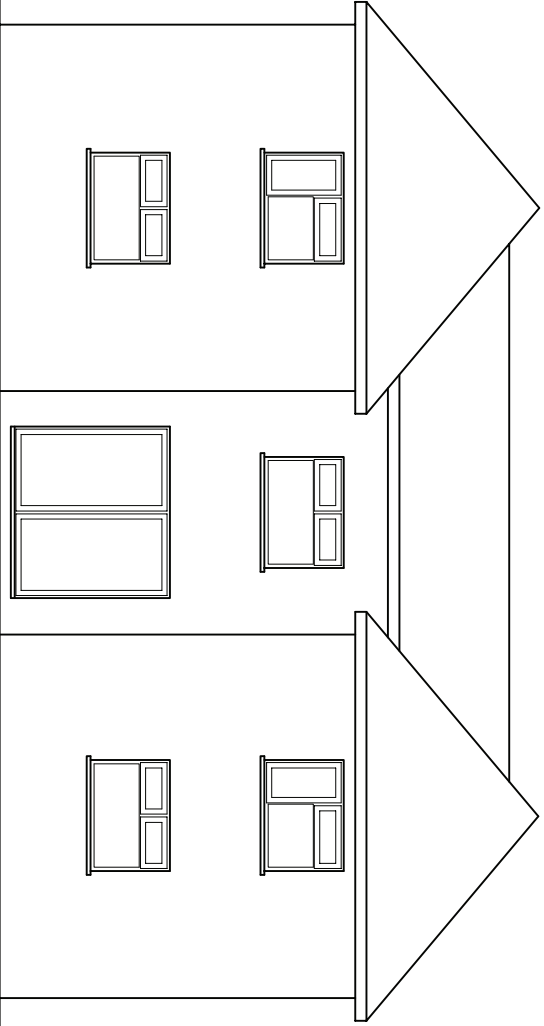
SOUTH ELEVATION
