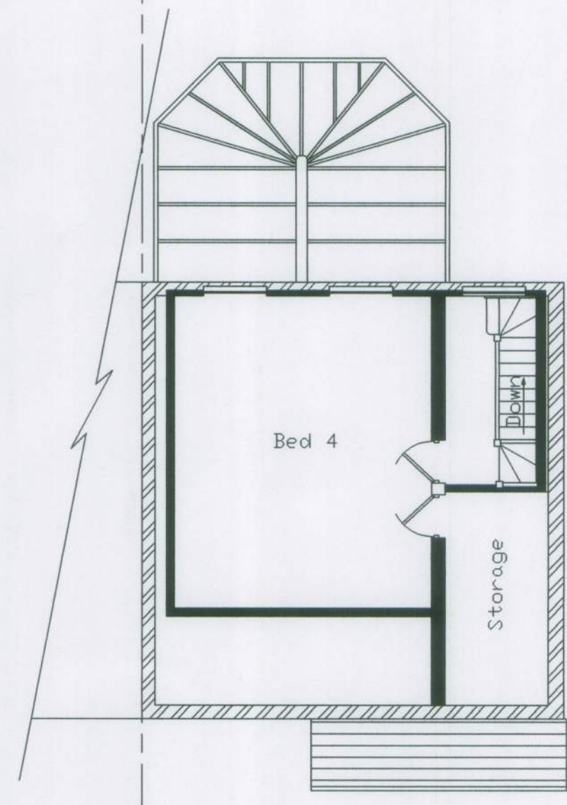
Proposed Loft Room Plan
