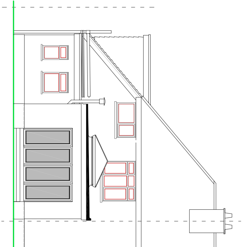
REAR ELEVATION
